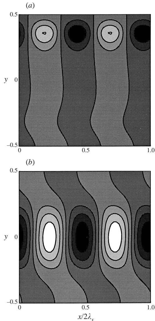
FIGURE 19. The solids fraction disturbance of the dominant modes at the points \oplus and \ominus in figure 17. (a) \bar{v} = 0.30 , H = 50 , k_x = 0.015 ; (b) \bar{v} = 0.55 , H = 50 , k_x = 0.013 . The patterns must be stretched by factors of 840 and 965, respectively, in the x -direction to view their true aspect.
