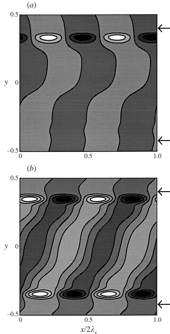
FIGURE 21. The solids fraction disturbance of the dominant modes in figure 20. Panel (a) is the (forward propagating) travelling instability corresponding to the second peak in the growth rate of figure 20 and panel (b) is the strong stationary wave instability corresponding to the third peak. The arrows in each panel indicate the locations where the base-state solids fraction is 0.649.
